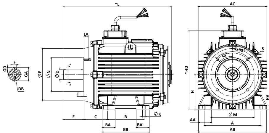
FOOT MOUNTED AND FLANGED MOTOR (FORM "C" - IEC 60072-1) - B34
