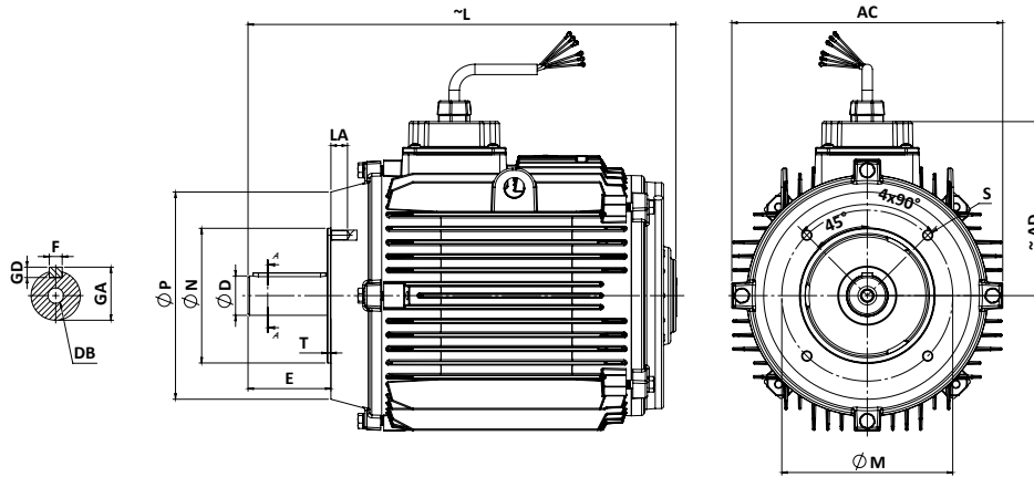
FLANGED MOTOR (FORM "C" - IEC 60072-1) - B14, V18, V19
